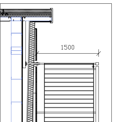
GALVANISED STEEL BALUSTRADE TO ROOF
