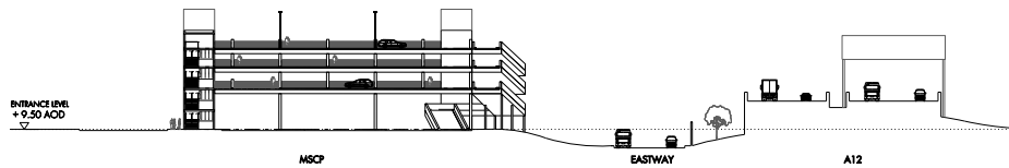
03 SECTION 03
