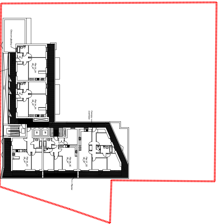
FIFTH FLOOR
