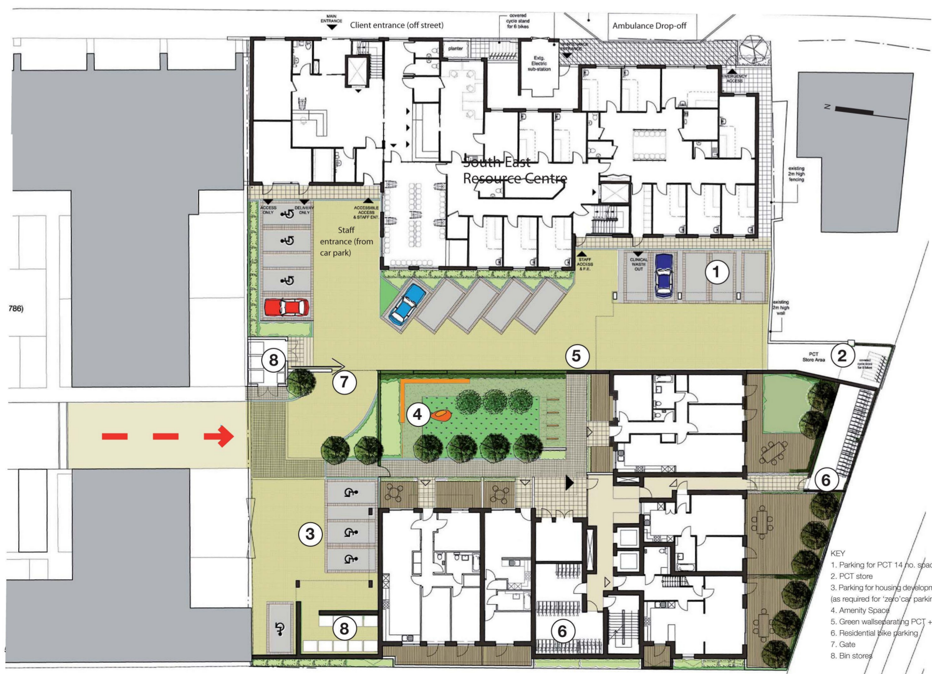
Ground Floor Plan (L1)
